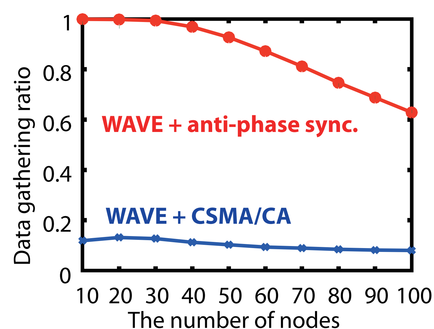
Data gathering ratio against the number of nodes
