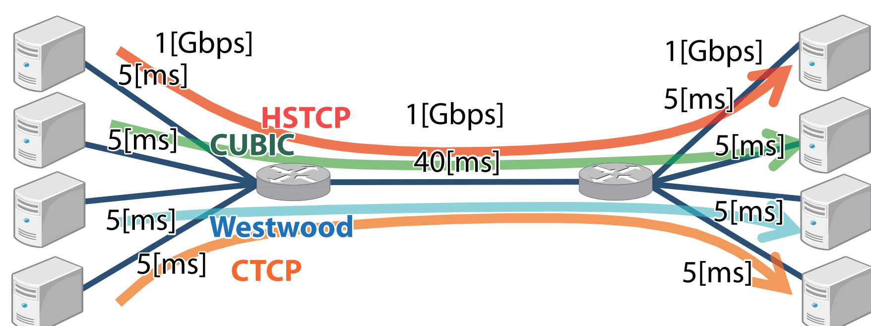
Figure 4: Simulation environment
