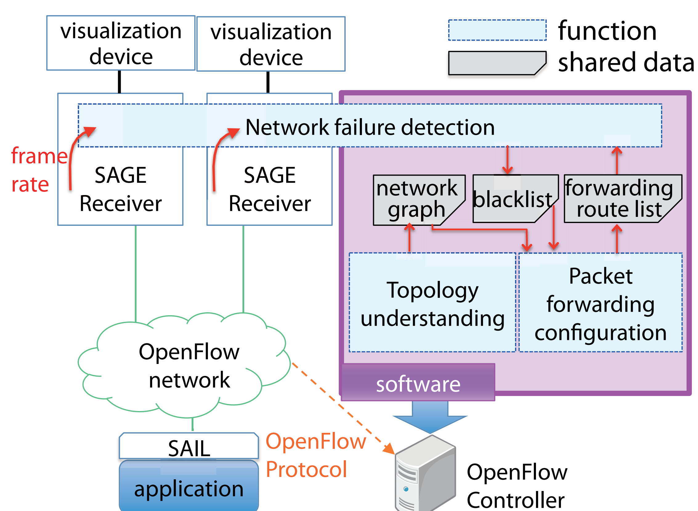
Fig.3 Proposed functionality
